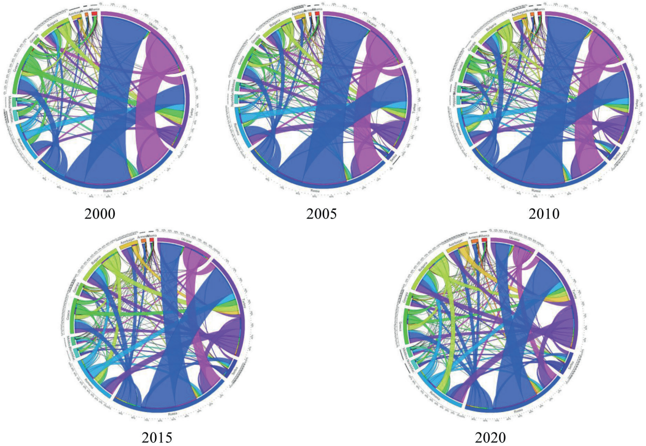
Figure 1. Results of visualizations, generated using the tableviewer utility script in Circos according to Gravity Model
